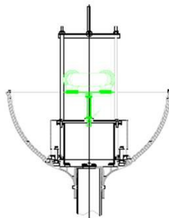
3. MONTAR BOMBILLA
