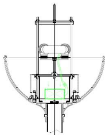
4. COLOCAR DRIVER Y CONECTAR
